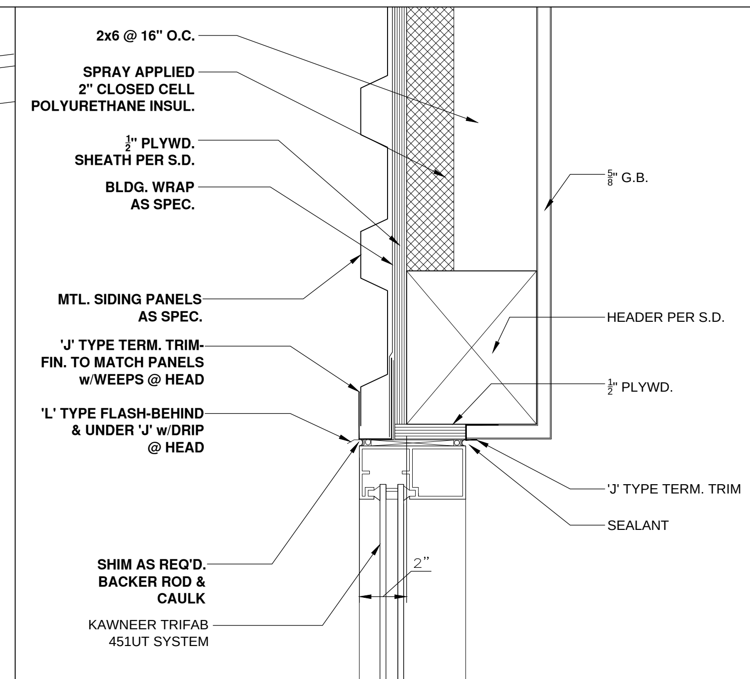
10 HEAD DETAIL /JAMB SIM.
