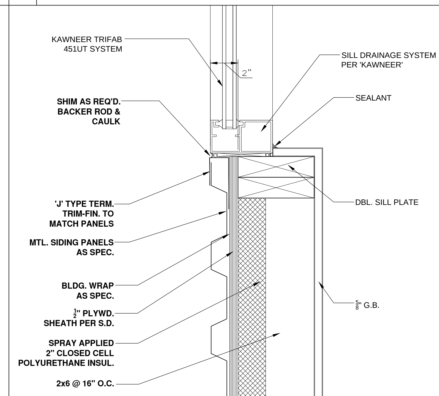
6 SILL DETAIL
