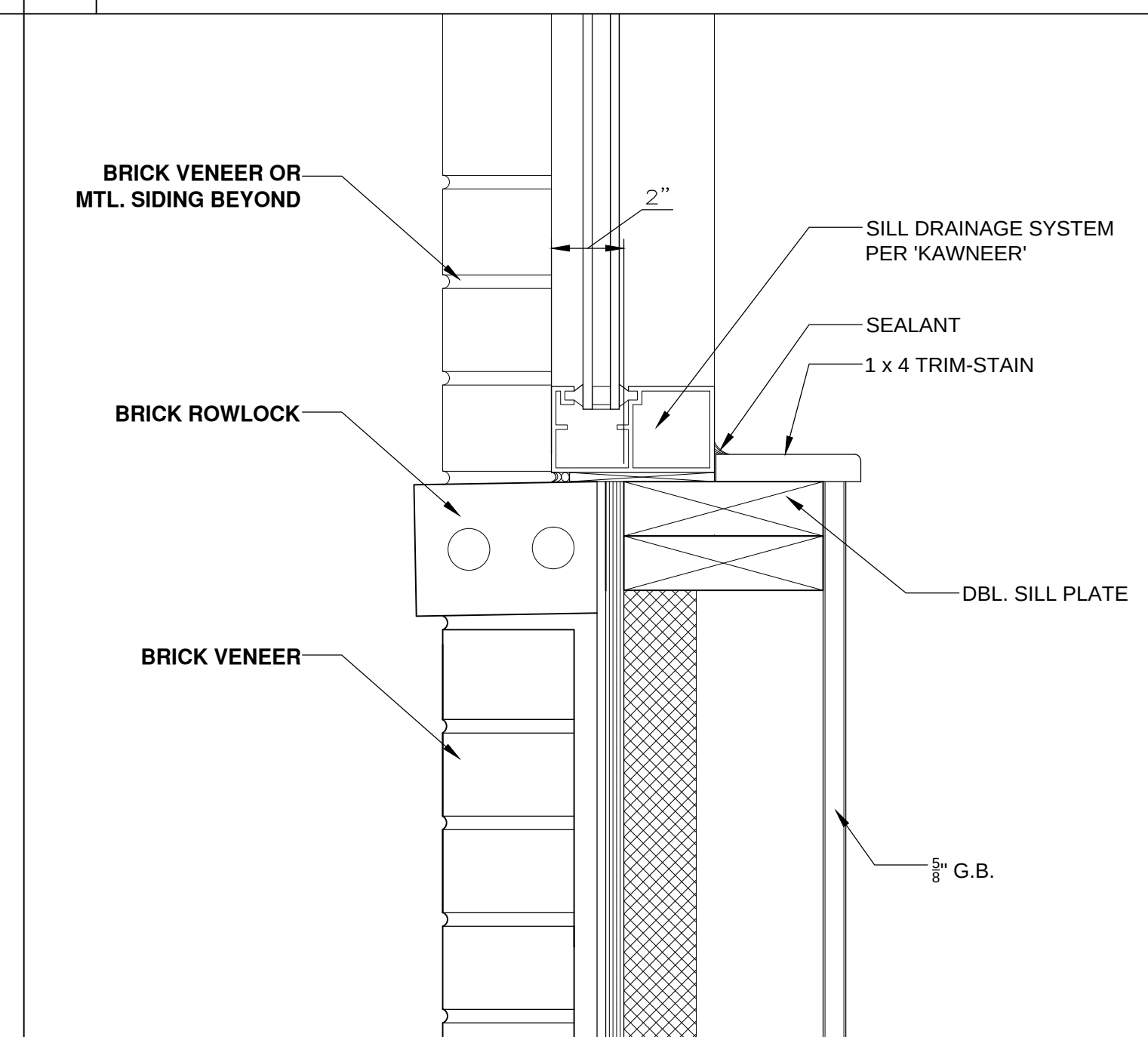
5 SILL DETAIL
