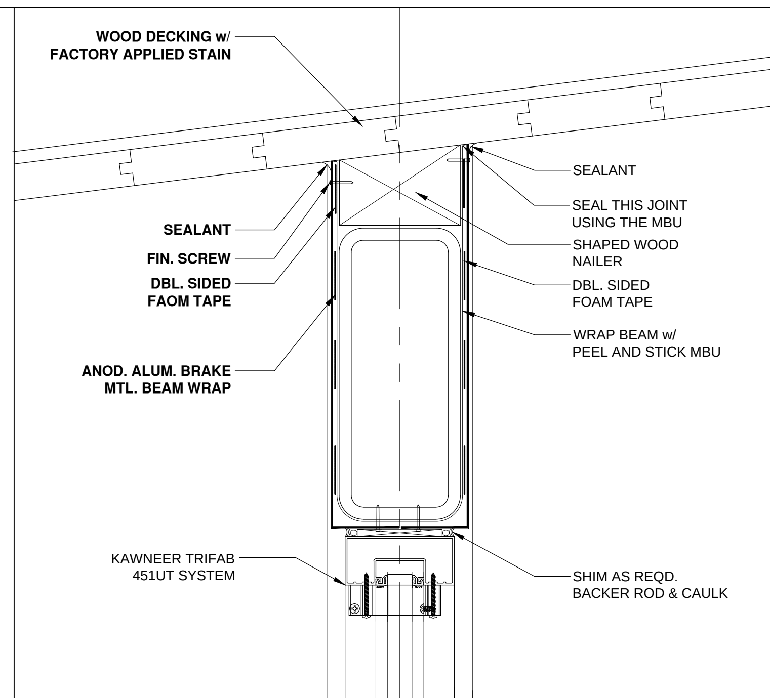
11 HEAD DETAIL
