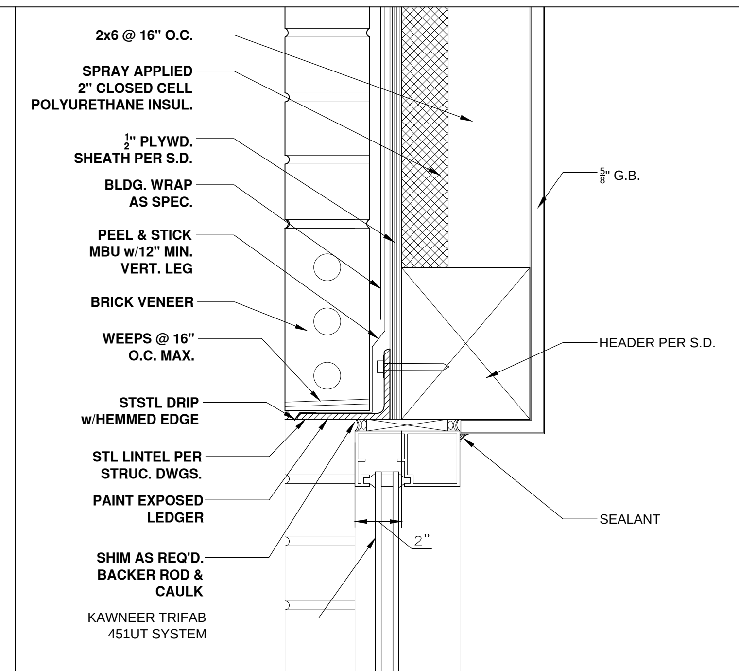
9 HEAD DETAIL
