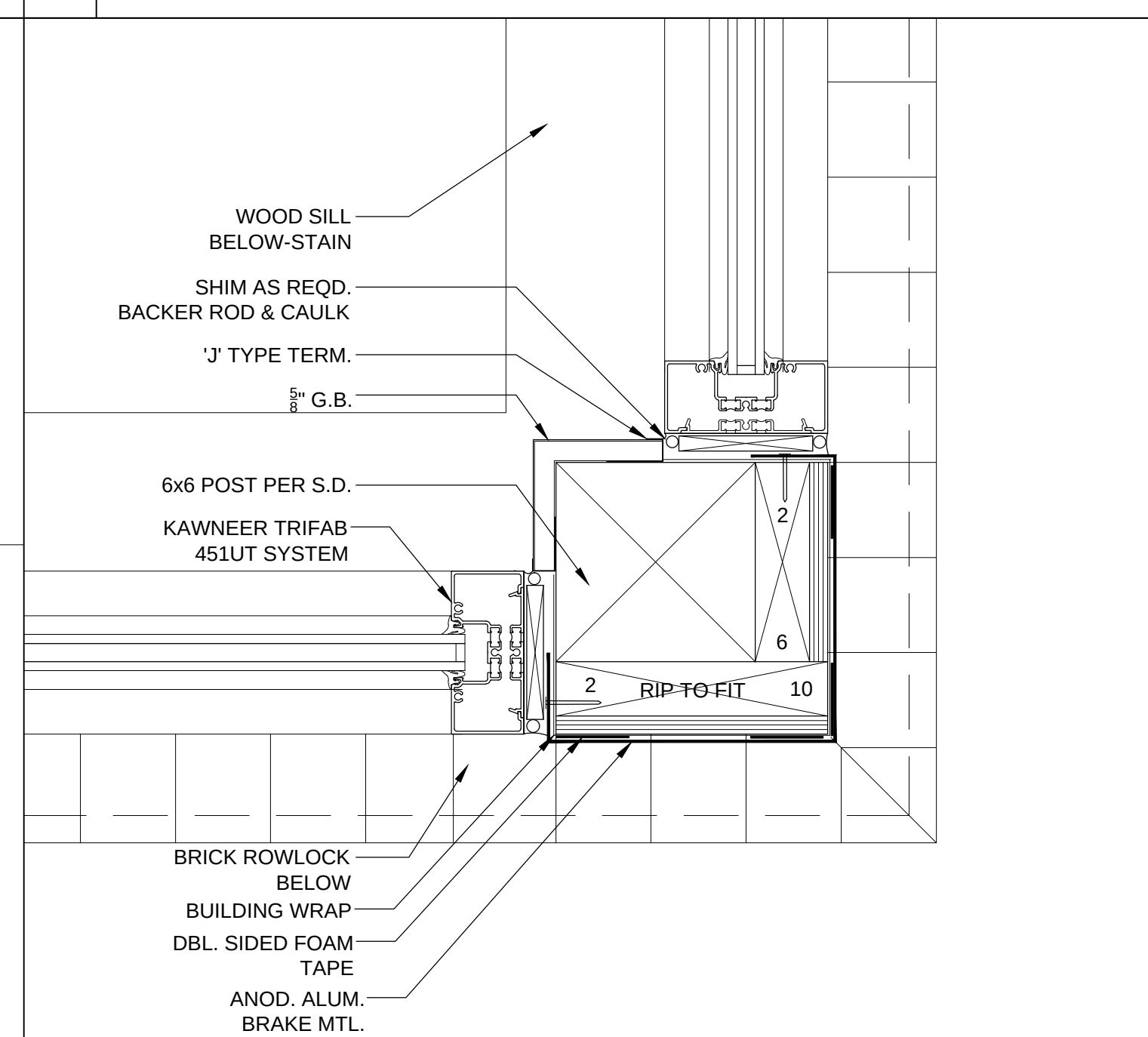
1 JAMB DETAIL / HEAD SIMILAR
