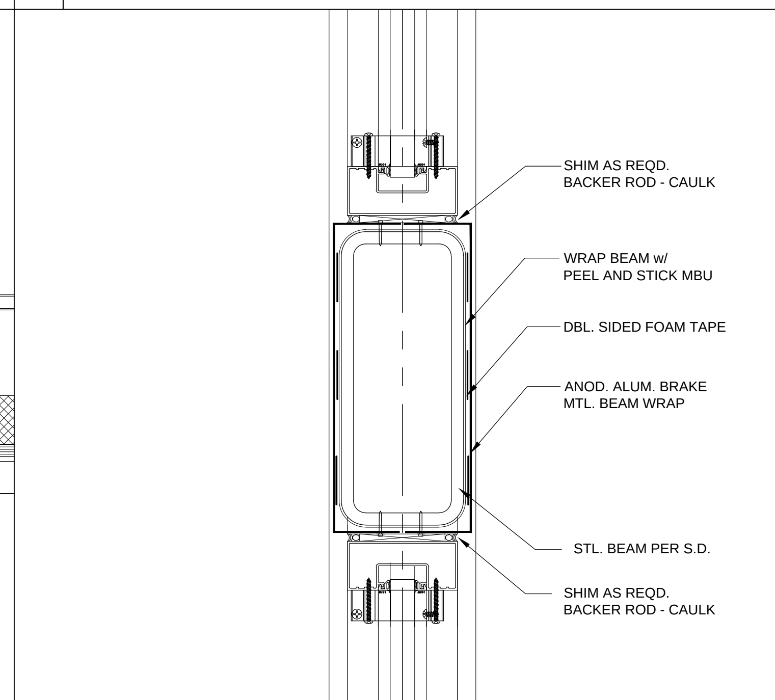
7 HEAD / SILL DETAIL
