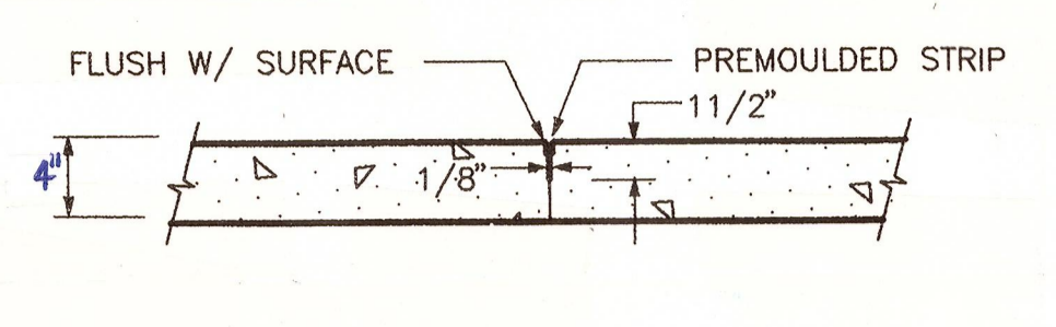
2 CONCRETE SIDEWALKS 3/4" = 1'-0"
