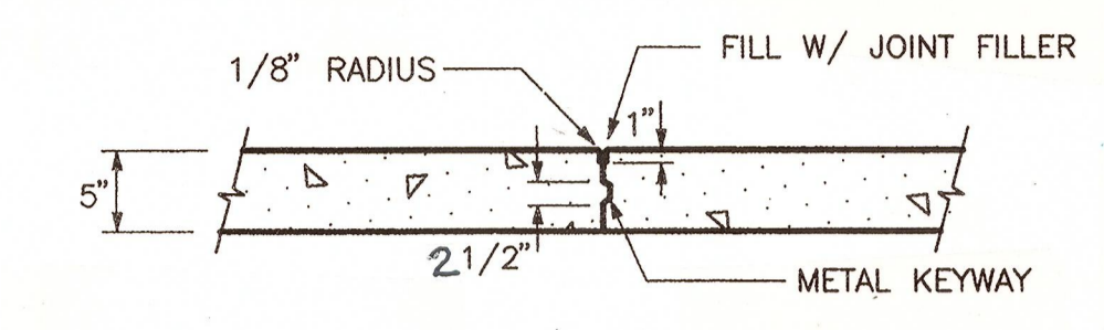
1 CONCRETE DRIVEWAY AND PARKING AREAS 3/4" = 1'-0"
