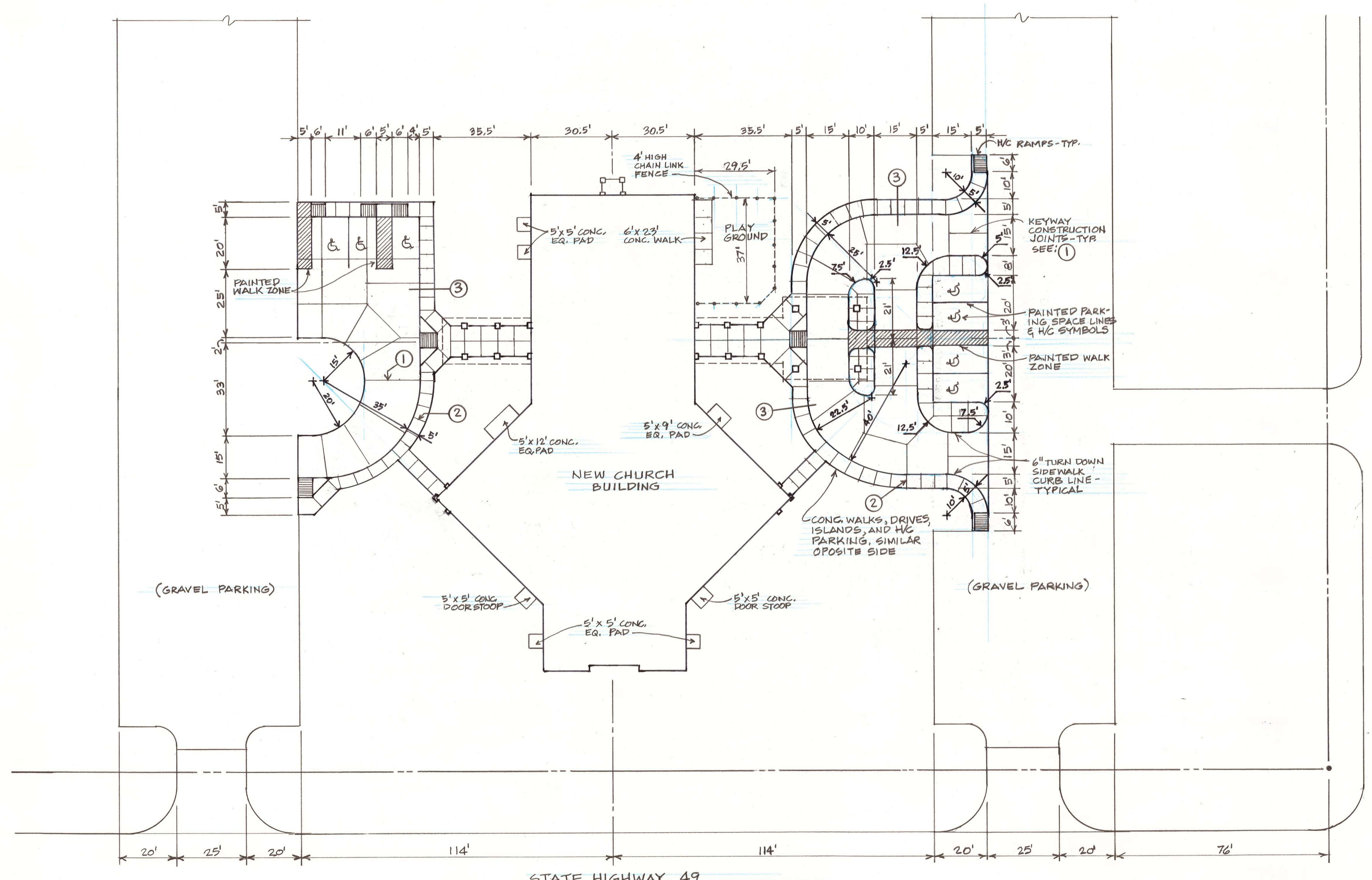
SITE IMPROVEMENTS PLAN SCALE: 1" = 20'
