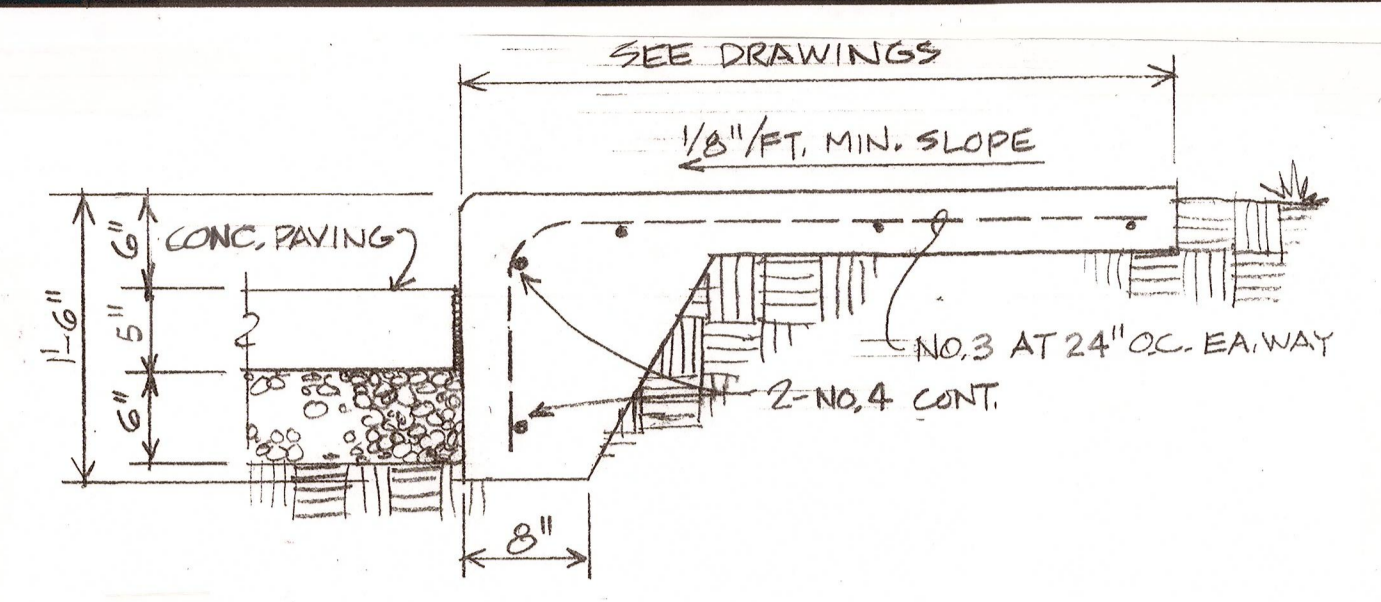
3 COMBINED CURB AND WALK 1" = 1'-0"
