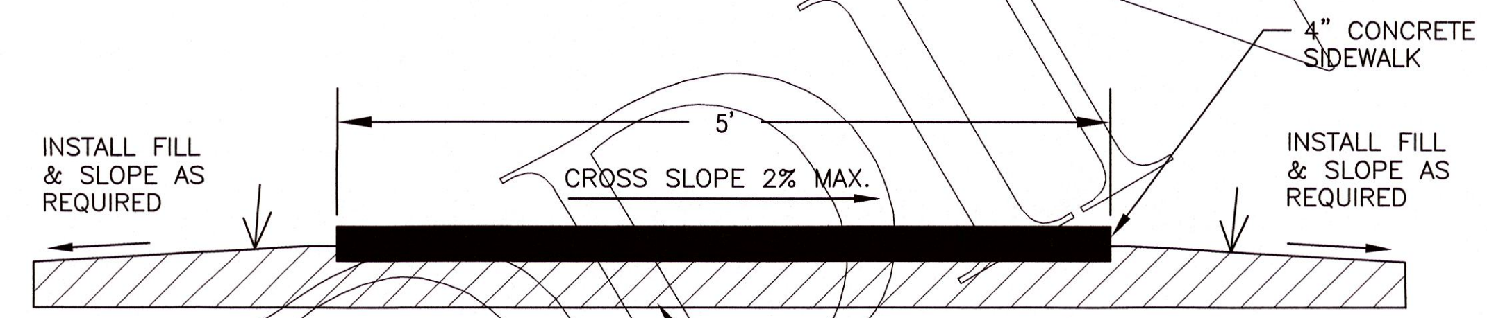
PLAY STRUCTURE FOOTING DETAIL (NIC) N.T.S.
