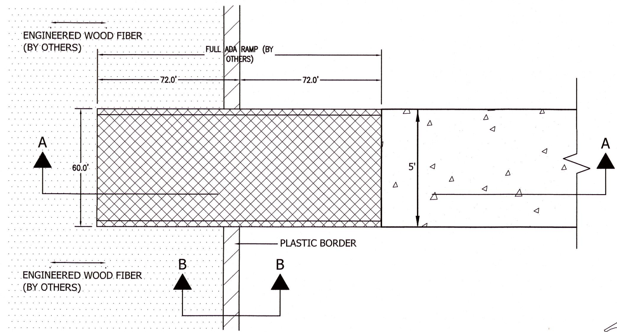
PLAN AT ADA RAMP N.T.S.
