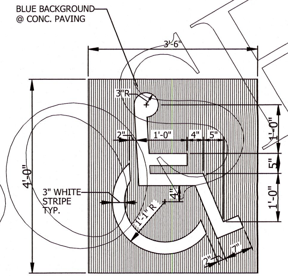
ADA PARKING STALL SYMBOL N.T.S.
