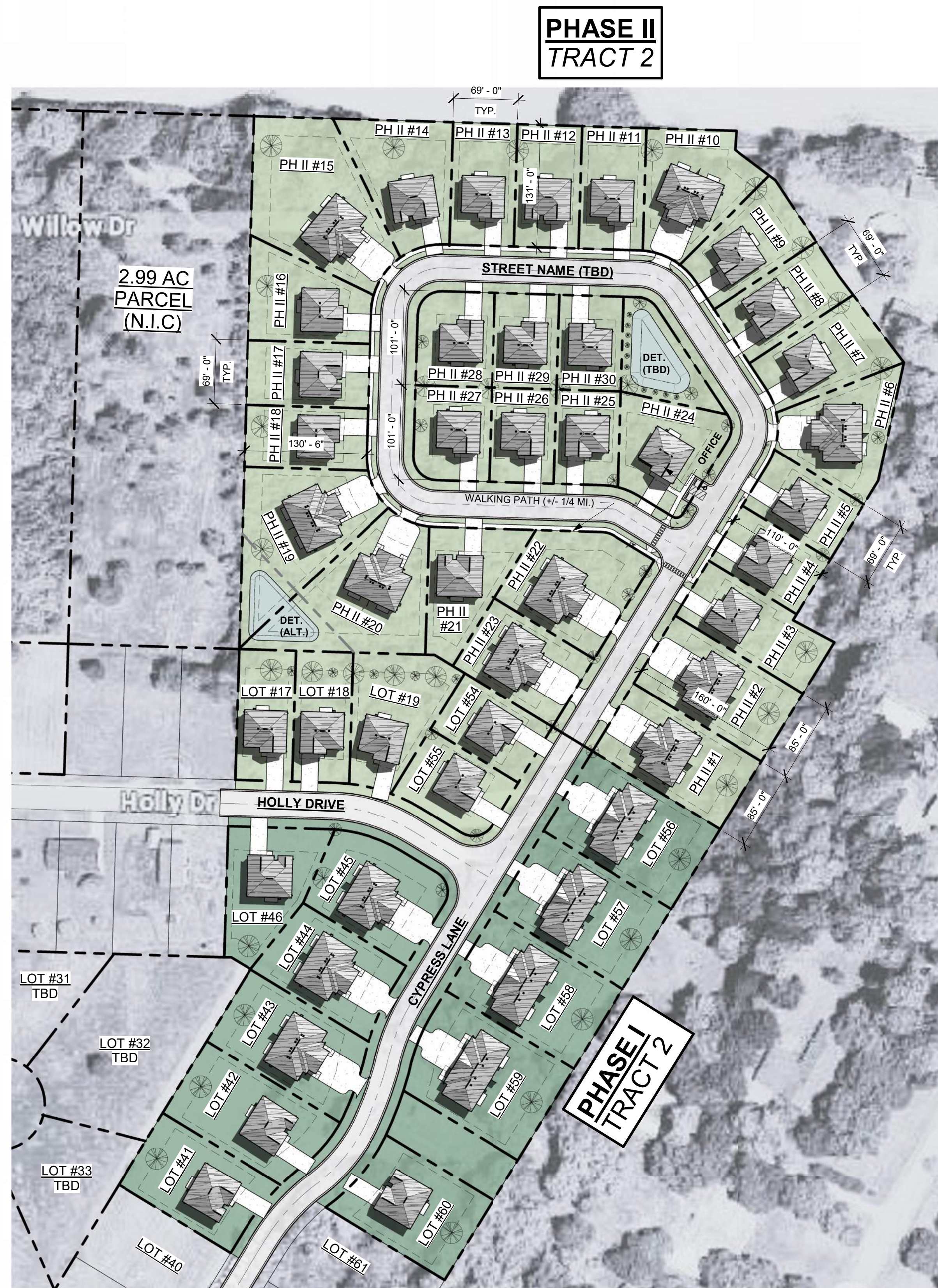
1 CONCEPTUAL SITE PLAN (PHASE I & II)
