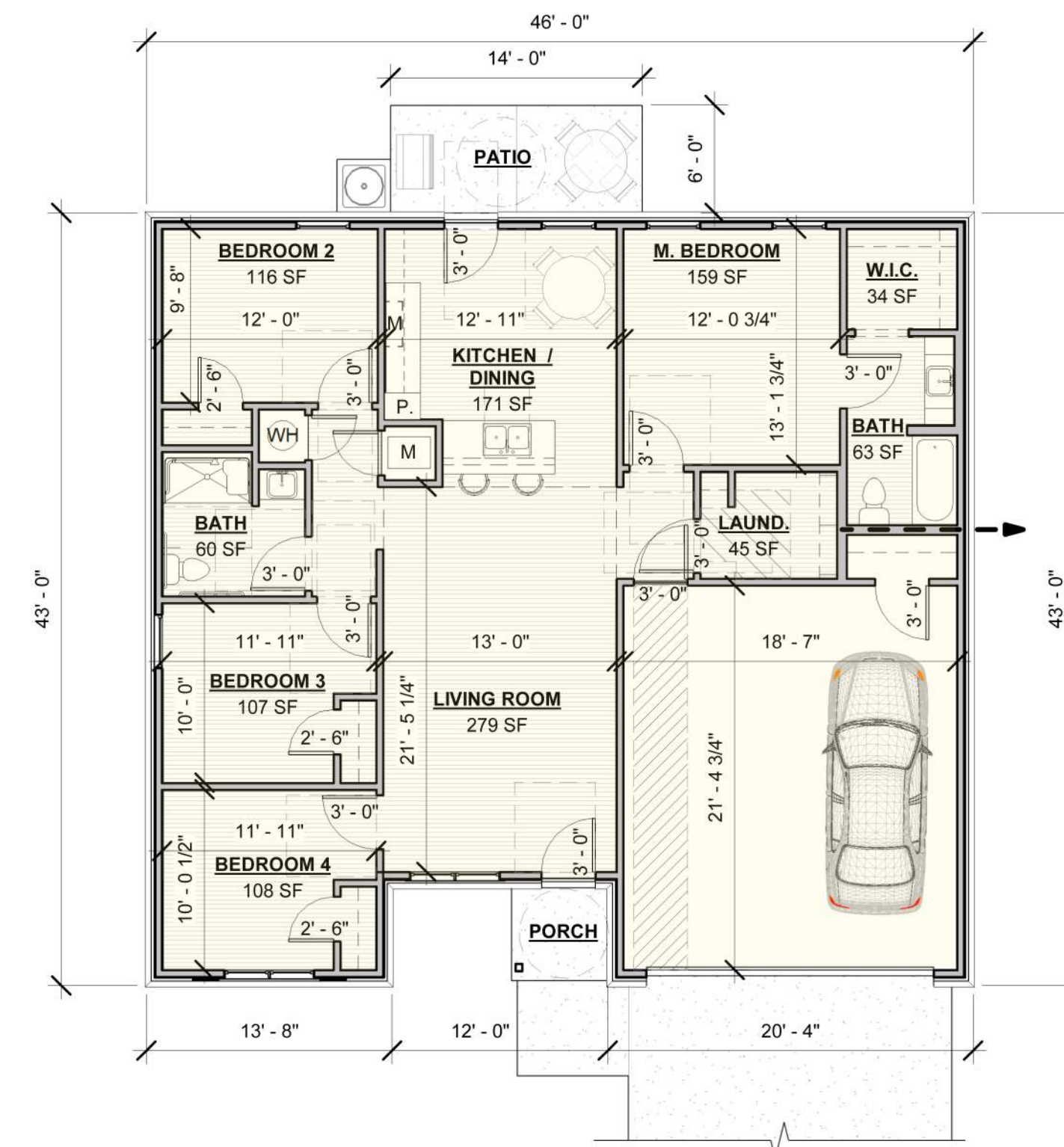
1 SGL. FAM. - 4 BEDROOM 1/8" = 1'-0"
