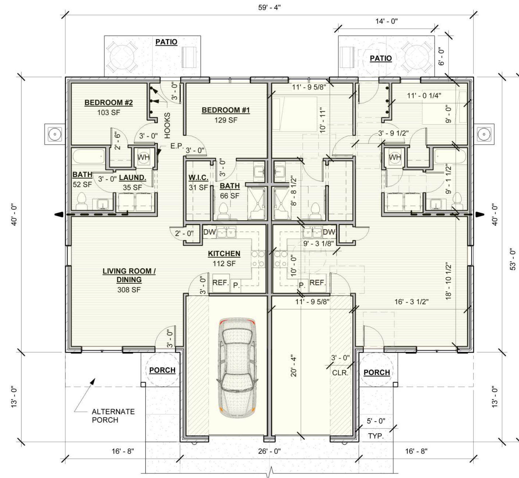
1 DUPLEX - 2 BEDROOM 1/8" = 1'-0"
