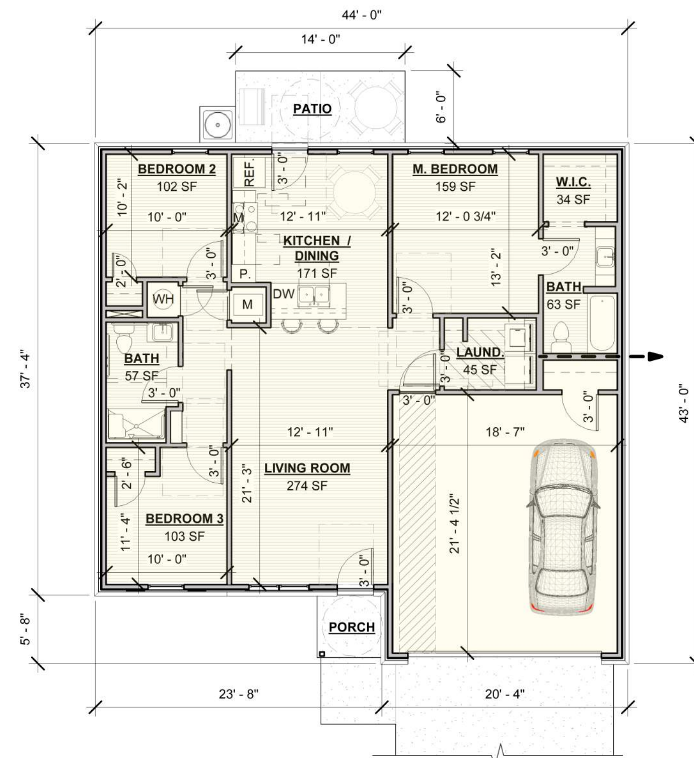
1 SGL. FAM. - 3 BEDROOM 1/8" = 1'-0"
